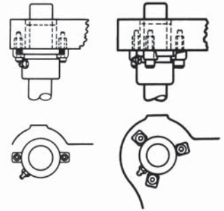
CLAMP ASSEMBLY FOR DEMOUNTABLE BUSHINGS
