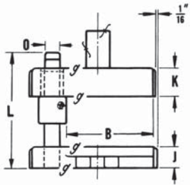
CLAMP ASSEMBLY FOR DEMOUNTABLE BUSHINGS
