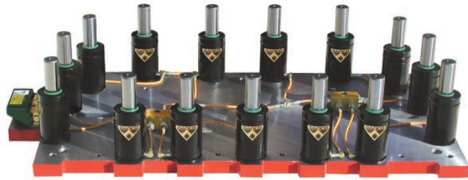
DADCO SMS® with fifteen 90.9.01500 cylinders linked using 90.700 (Y-700) hose with permanent hose adapters. This system employs two distribution blocks to simplify piping to a mini control panel that is used to drain, fill and monitor the pressure from outside the die. Contact DADCO for more information on linked operations.
